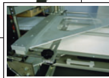
"APA" Automatic product size adjustment of inverting triangle & infeed conveyor * Exclusive feature!
